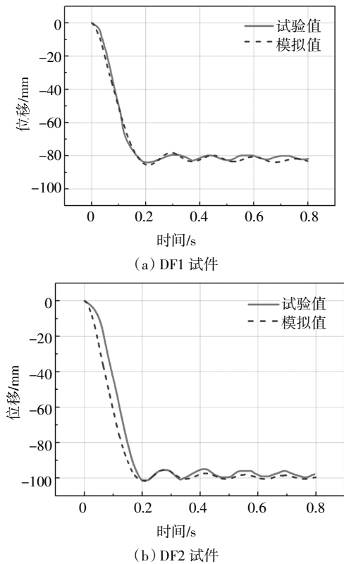
图8 DF1和DF2试件试验与模拟角柱竖向位移对比 Fig.8 Comparison of vertical displacement between DF1 and DF2
