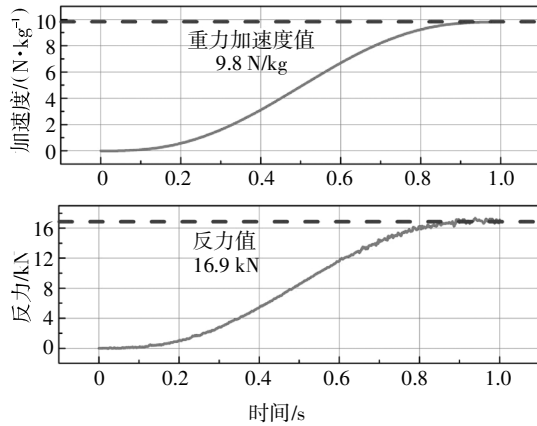
图6 荷载加载曲线 Fig.6 Loading curve
