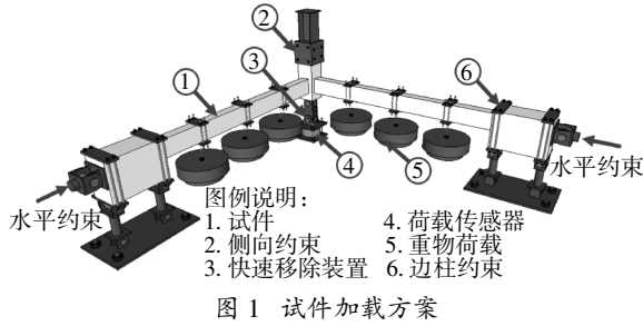
Fig.1 Specimen loading scheme
