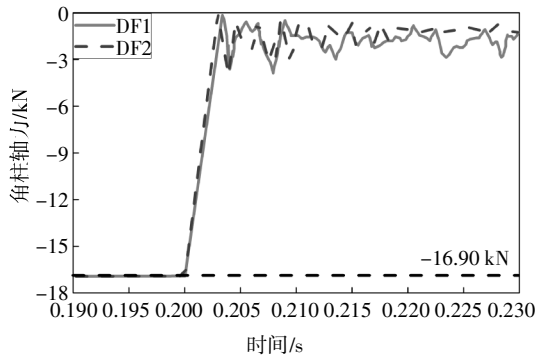
图 2 角柱轴力释放过程 [3] Fig.2 Axial force release process of corner column
