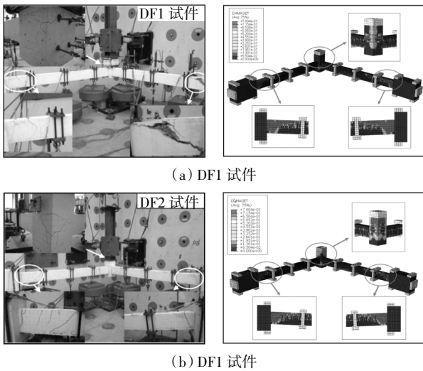
图9 试件破坏形式与模型受拉损伤对比 Fig.9 Comparison of failure mode between field test and finite element model
