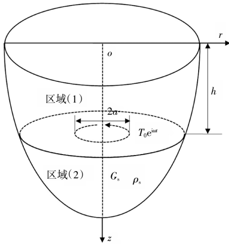
图 1 饱和地基中埋置简谐扭转荷载简化分析模型 Fig.1 Simplified analysis model of buried torsional load in non-homogeneous saturated soil
